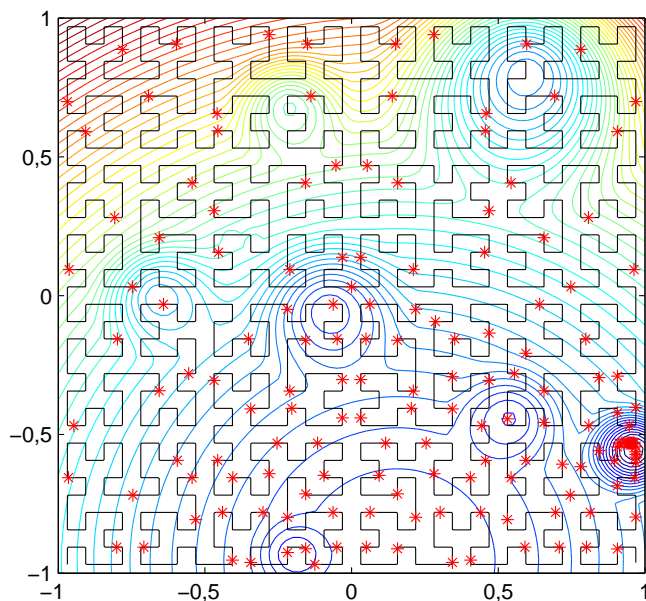
Figure 7: Trial points produced by the MGAS and Peano curve approximation of level 5 while optimizing Function no. 6, class 1, generated by the GKLS-generator; Table 1 describes this and other classes of test functions used in the numerical experiments.
