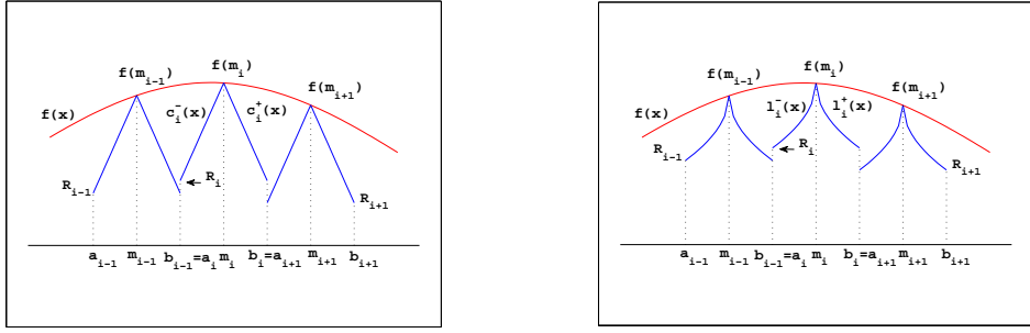
Figure 2: Lipschitz (left) and Hölder (right) support functions.
